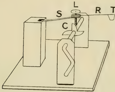
FIG. 10.—THE SPRING-TAPPER
