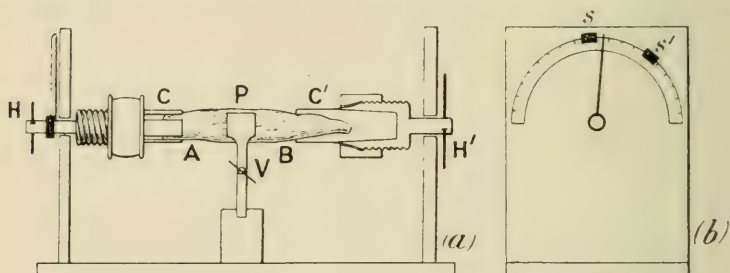
FIG. 11.—THE TORSIONAL VIBRATOR
