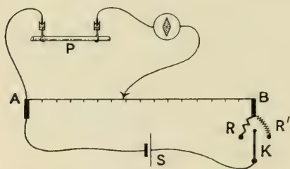
FIG. 9.—THE COMPENSATOR
